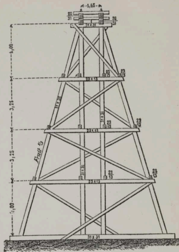
46. Виадукъ Central Pacific.
